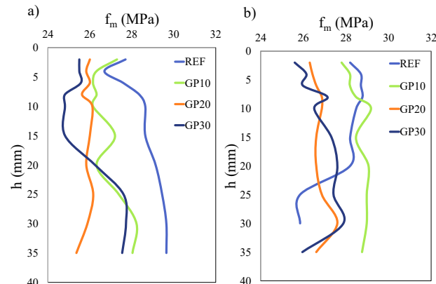
Fig.6 Calculated compressive strength relative to sample height for mortar: a) air-cured overlays, b) humid-cured overlays
