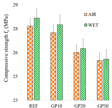
Fig.5 Average compressive strength f_c of the subsurface layer.
