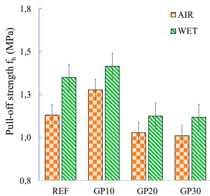
Fig.4 Average pull-off strength f_h of the subsurface layer.
